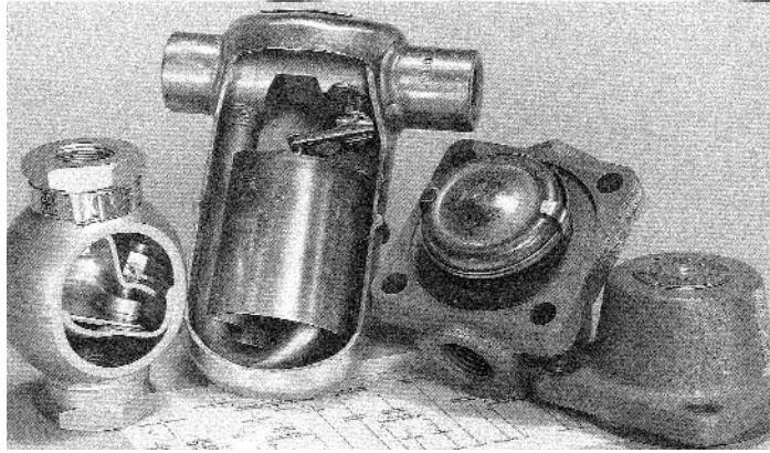
L to R - Adjustable Bimetallic trap, Inverted Bucket trap, Balanced Pressure Thermostatic trap
