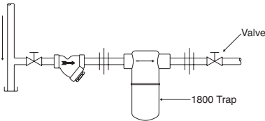
Fig. 4-2. Hookup for No. 1800 Series Stainless Steel trap.
