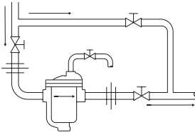
Fig. 5-1. Bypass hookups for No. 800-816 and 880-883 traps.
