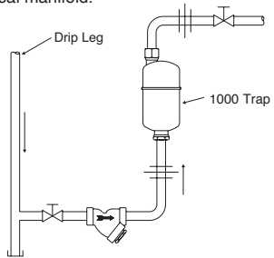
Fig. 4-3. Hookup for No. 1000 Series Stainless Steel trap.
