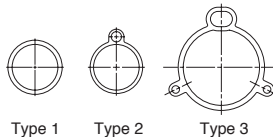
Fig. 27-2. Gasket Types
