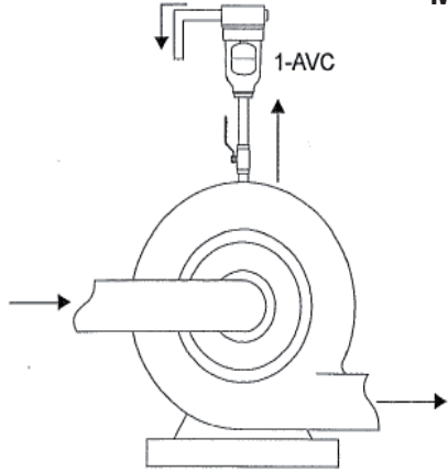
Figure 3 Automatic air vent on centrifugal pump. A full ported 3/4" valve and pipe must be used.
