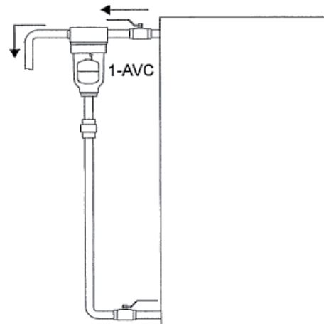
Figure 2. Automatic air vent discharging surplus air from water storage tank. Note: Remove plug from cap in this installation.
