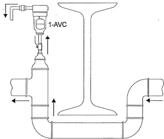
Figure 7 Automatic air vent on loop in piping. A full ported 3/4" valve and pipe must be used.
