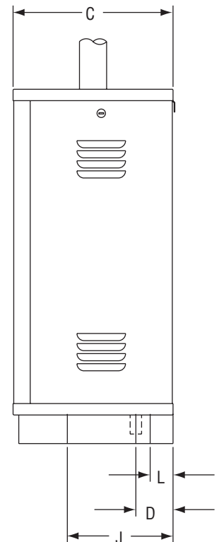
Figure 145-5. Model EHU-703 and 704 — Side View
