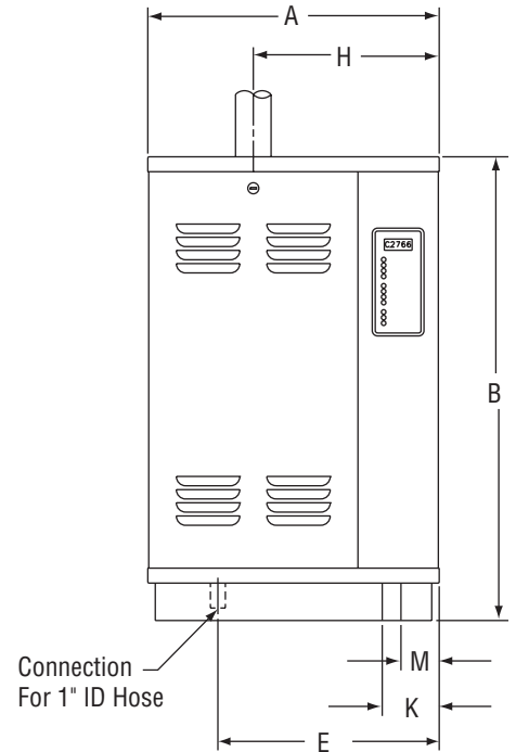
Figure 145-3. Model EHU-703 — Front View
