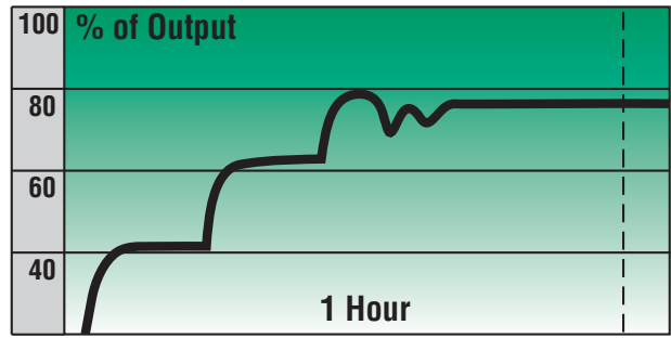
Chart 138-1. This chart represents the patented self-regulating maximum output of the EHU Series from start-up. To avoid hunting, the unit gradually increases capacity from 40% of maximum to 60% to 80%. In this case, the output satisfies the humidistat demand at a level below 80% of maximum capacity. The modulating feature then takes over and controls the unit output. The self-regulating maximum output can then adjust up (to 100% in this example) or down (to 60%) as demand history warrants. The feature intermittently "resizes" the humidifier's maximum capacity to avoid hunting and to provide humidity control.
