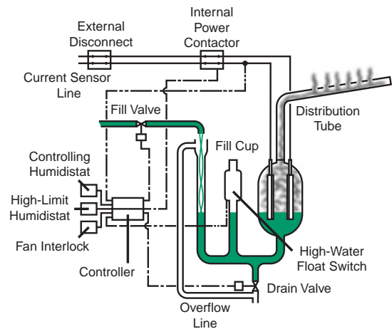
Figure 137-1. 100% demand. Filling with water. Low, increasing steam output.
