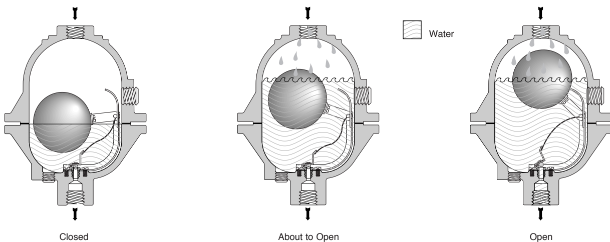
Figure LD-11. Operation of No. 71-A Snap Action Drain Trap
