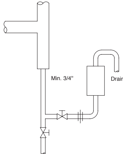
Figure LD-15. Series 200 or 300 inverted bucket drain traps installed on compressed air line contaminated by oil.
