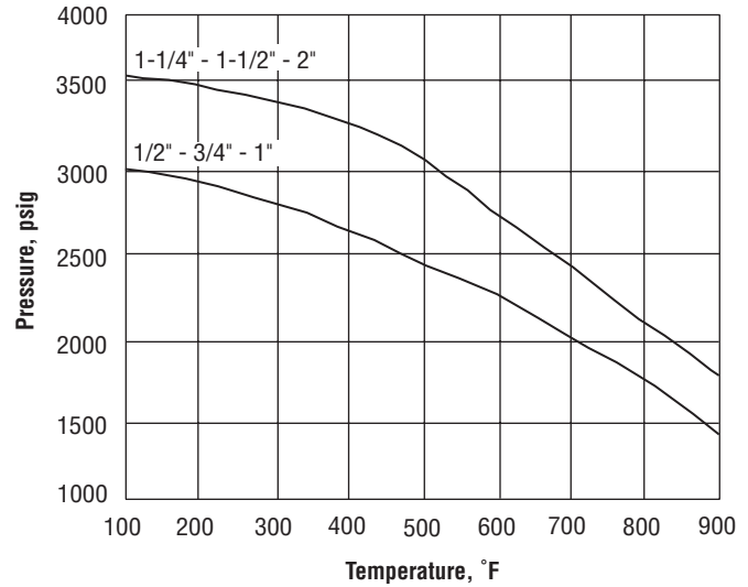
Pressure/Temperature Rating
