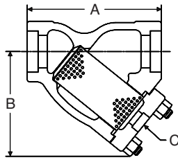
C1SC/C1SW 1-1/4", 1-1/2", 2"
